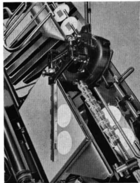
Group 50 Device for printing circular and oval disks with diameters of 1\frac{1}{2} to 4\frac{3}{4} inches. Designed for two-up feeding.
